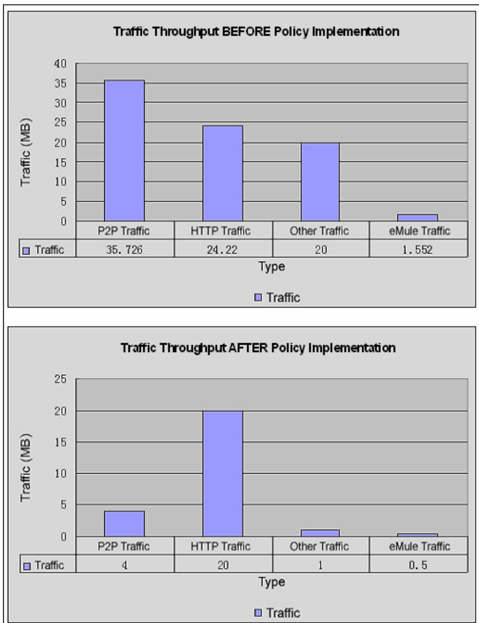
Figure 8: Effects of Traffic Management Policy Implementation
