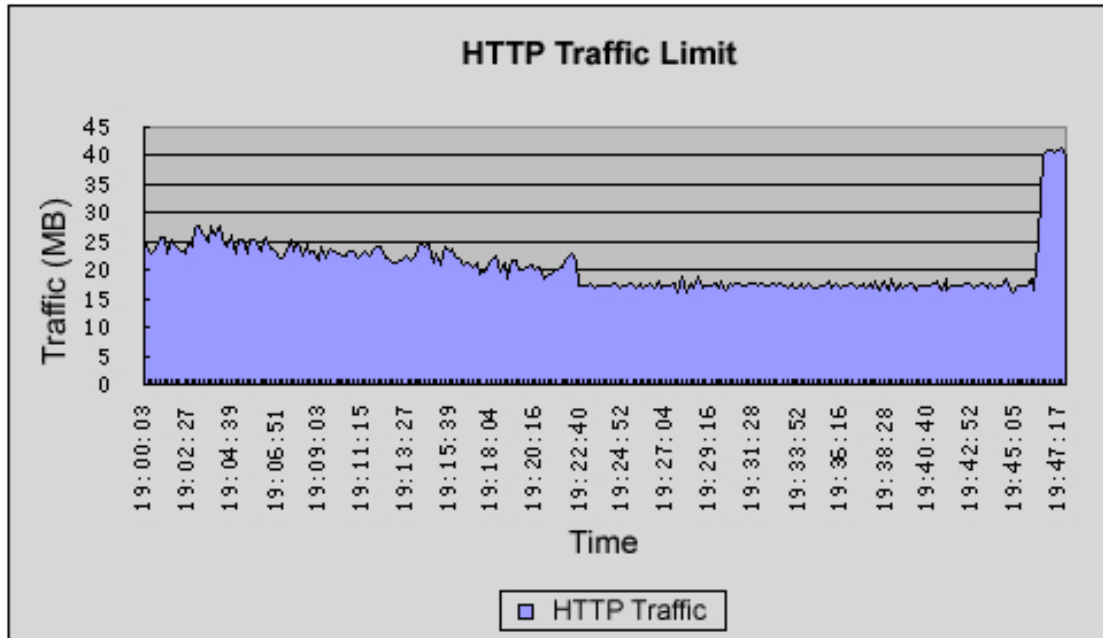
Figure 6: HTTP Traffic Limit
