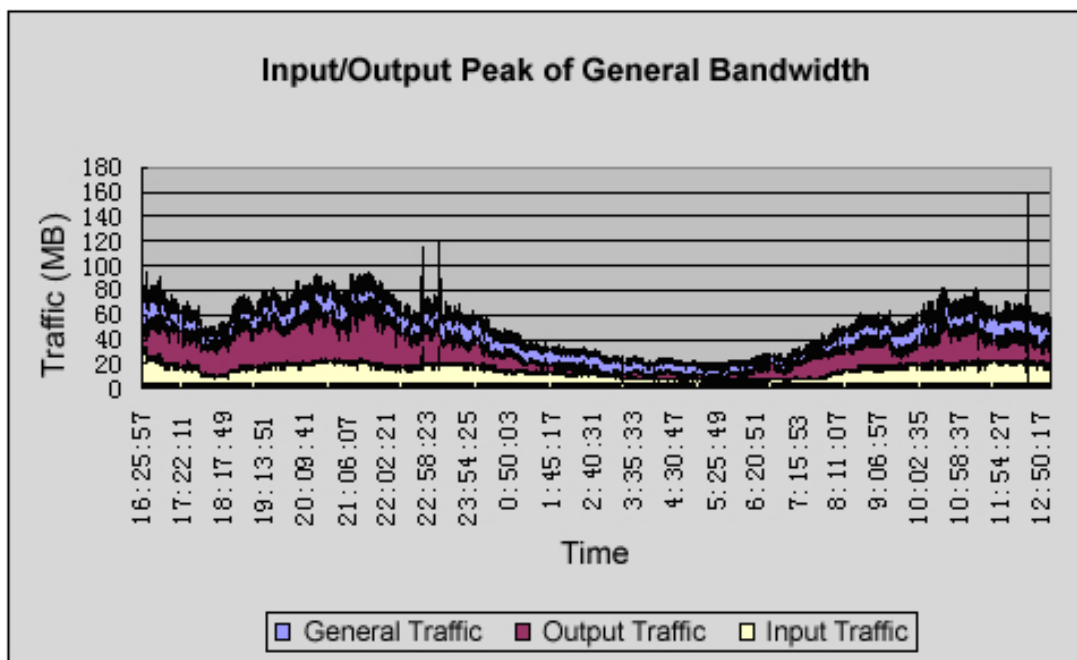
Figure 3: Input/Output Peak of General Bandwidth
