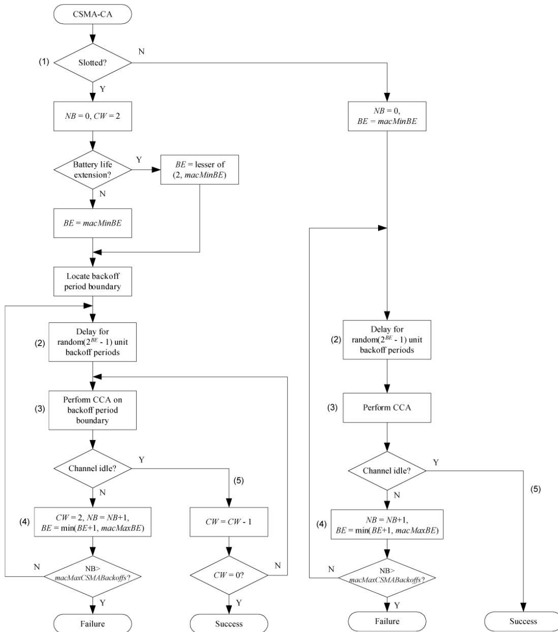
Figure 69—CSMA-CA algorithm
