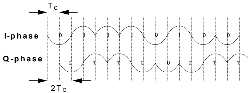
Figure 27—Sample baseband chip sequences with pulse shaping
